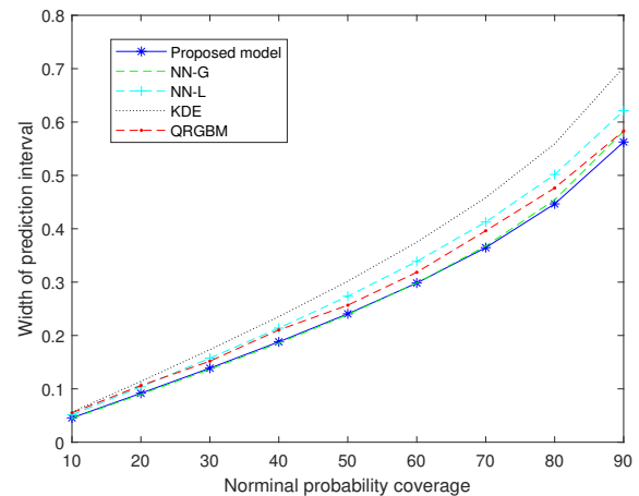
Fig. 6: Width of PI at wind farm 1
