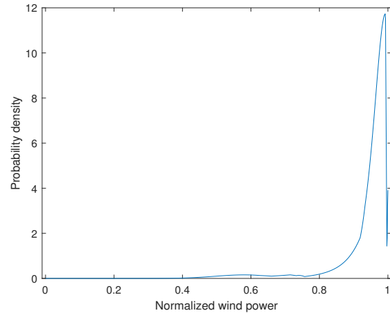
Fig. 4: Illustration of probability density of 100-th sample in test set
