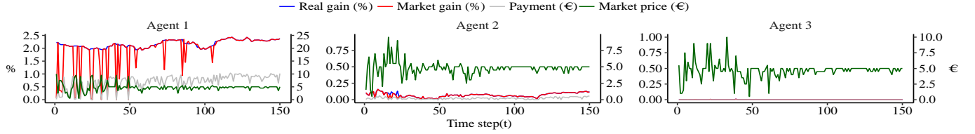
Fig. 5. Market dynamics for experiment E1 (bid price is constant and equal to 5€).
