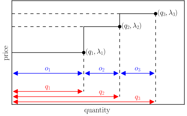
Fig. 1. An example offer curve with multiple blocks, which shows how market price scenarios are used as price offers, building an offer curve.
