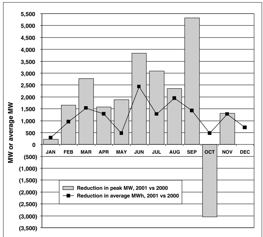
FIGURE 6 Reductions in electricity in 2001 and 2000. Source: Sweeney, 2002.
