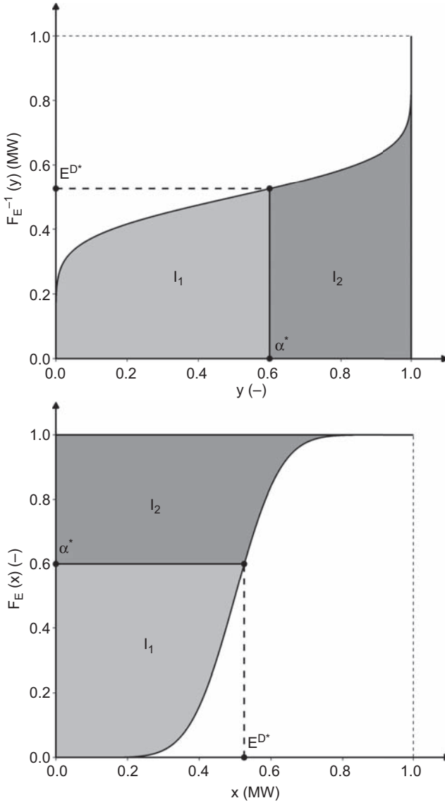
Figure 10.4 Integral form interpretation of EOL^*_{t+k} (\bar{E} = 1MW) .
